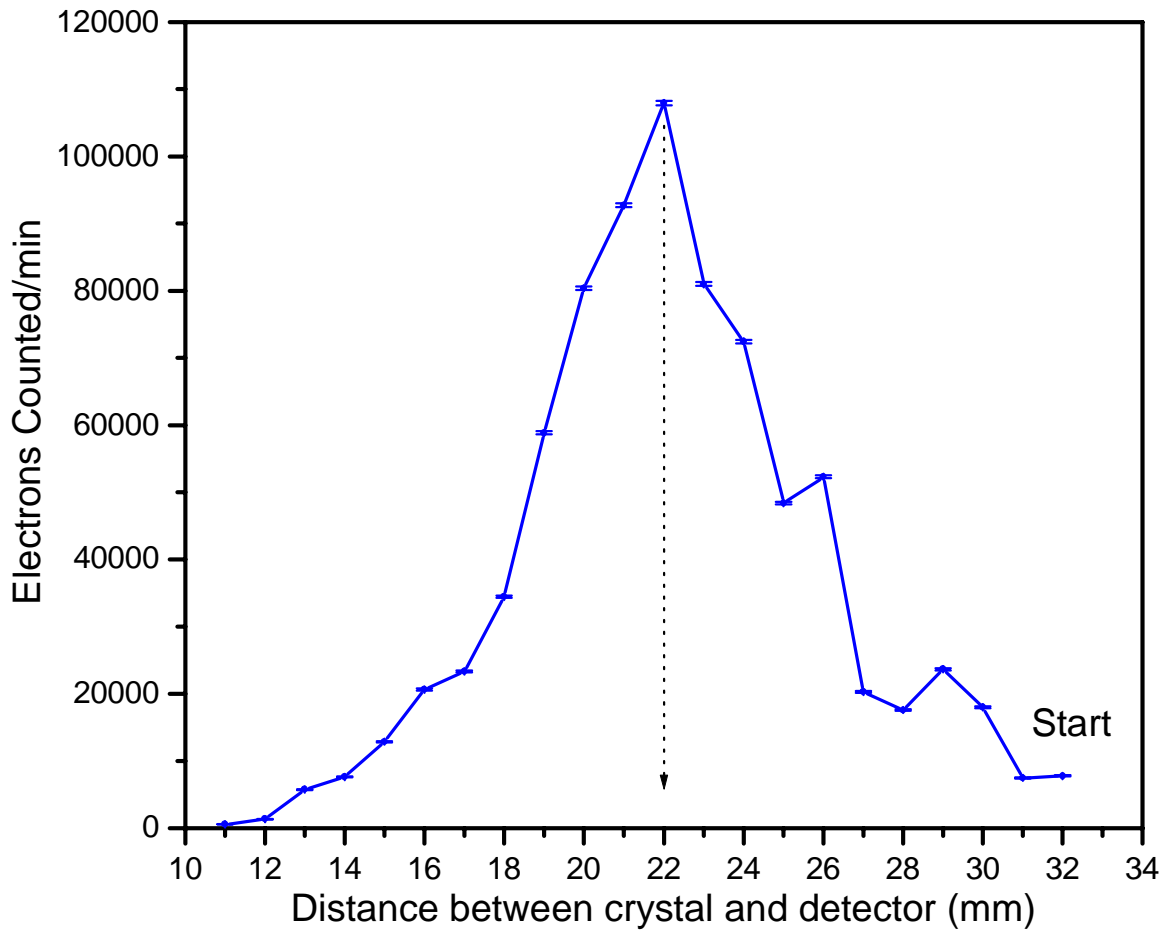
Beam profile as crystal is moved towards the detector in 1 mm increments.
