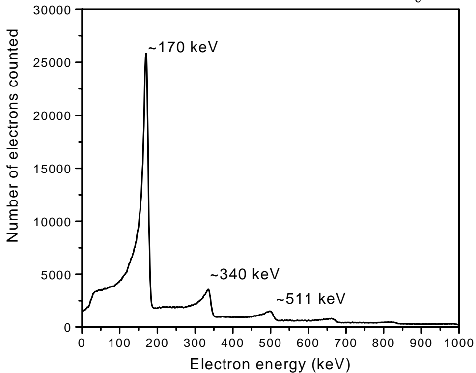
Electron spectra from a 4x10mm LiNbO 3 crystal
