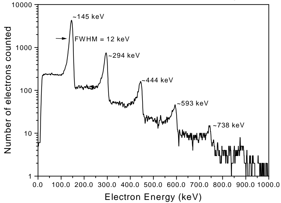
Electron spectra from a 4x10mm LiNbO 3 crystal
